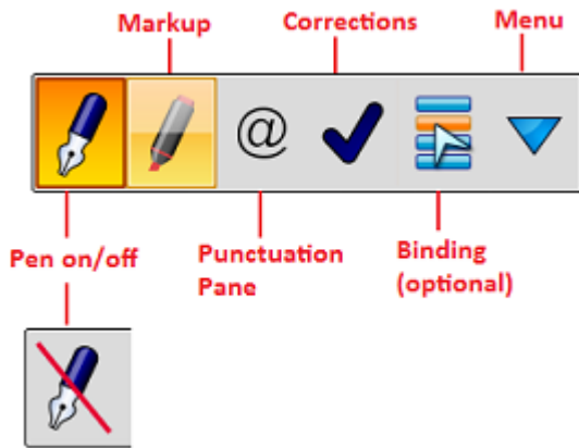
Main toolbar
